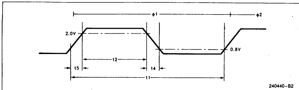
Figure 15.8. CLK2 Waveform
