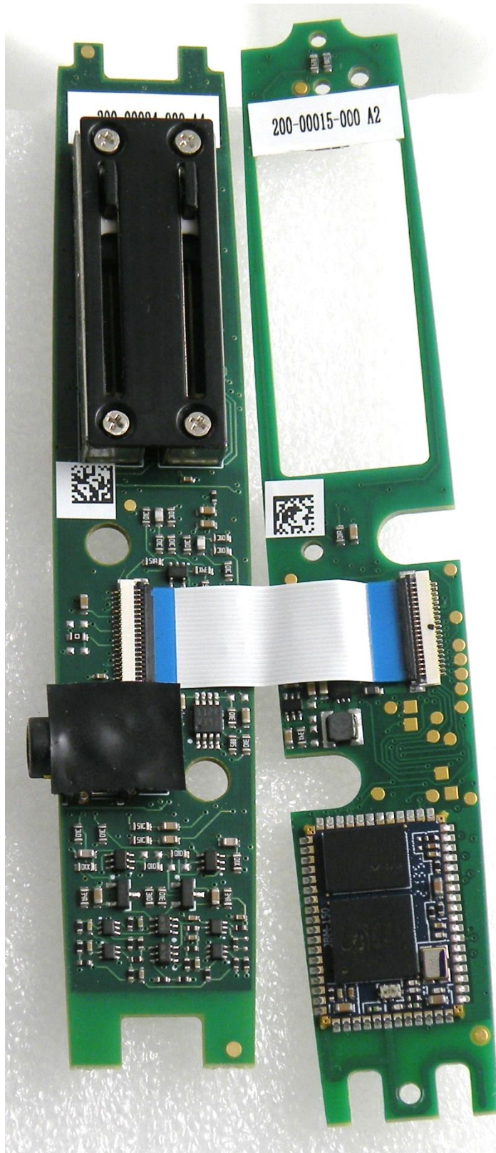
2:Control box PCBA's, "in" side
